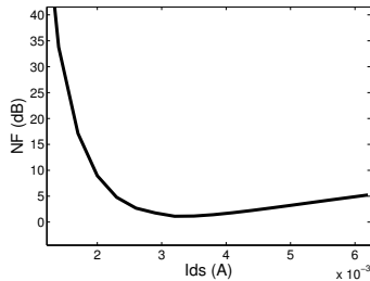
Fig. 3. The variation of the LNA Noise Figure in function of its biasing current. The Noise Figure is calculated using CAIRO+ and GiNaC for a 130nm CMOS process. ( V_{ds}=V_{gs}=0.6 V)
