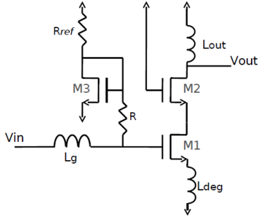
Fig. 2. The targeted circuit topology: cascode LNA with inductive source degeneration.
