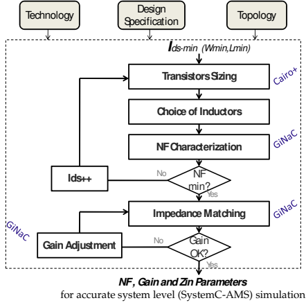
Fig. 5. Flow chart to implement the design and characterization method in a C++ environment
