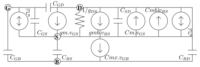
Fig. 4. The complete small signal MOS transistor model [12] (where: C_m = C_{dg} - C_{gd} , C_{mb} = C_{db} - C_{bd} and C_{mx} = C_{bg} - C_{gb} ), used in the proposed automatic synthesis and characterization procedure.
