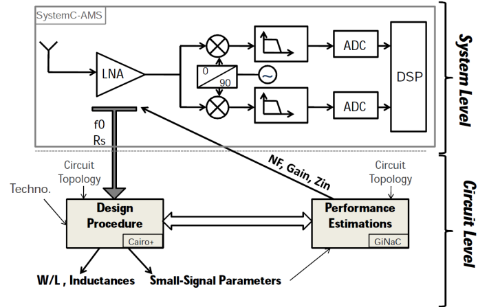
Fig. 1. The proposed C++ based environment for the automatic design and characterization of RF transceivers. (Simulation → SystemC AMS, Synthesis → CAIRO+, Characterization → GiNaC)
