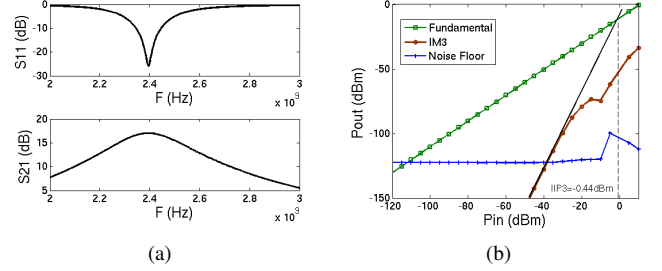
Fig. 7. Simulation results of the synthesized 2.4GHz LNA: (a) S_{11} , S_{21} and (b) IIP3 at f_0 = 2.4\text{GHz} .
