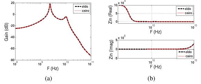
Fig. 6. Perfect matching between simulation results and the automatically characterized SystemC AMS models of the synthesized 2.4GHz LNA (a) Gain (b) Input Impedance.
